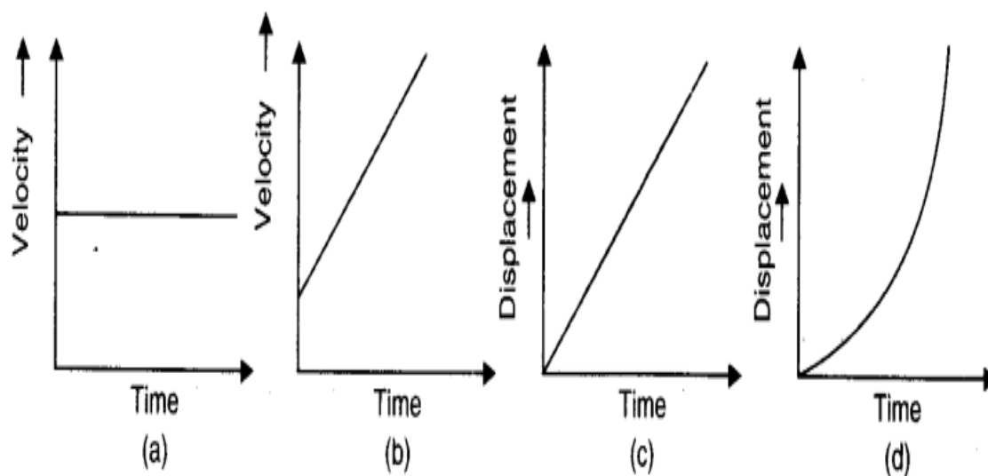
Fig. Curves (a) and (c) represent motion with a constant speed u . Curves (b) and (d) represent motion with a uniform acceleration a starting with an initial speed u .
